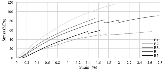
Fig. 18. Stress vs. strain curves for specimens B1-B5 under four-point bending test at 25 °C.
